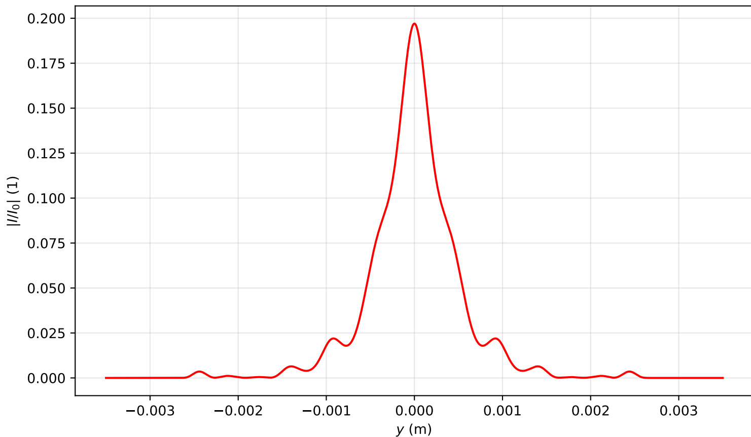
Intensity profile I(x=0, y, z=3.184)/I_0 , \text{Pin}=5.0\text{Pcr} , artificial time
